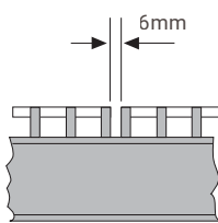
相鄰格柵間隙 Clearance between adjacent grating
